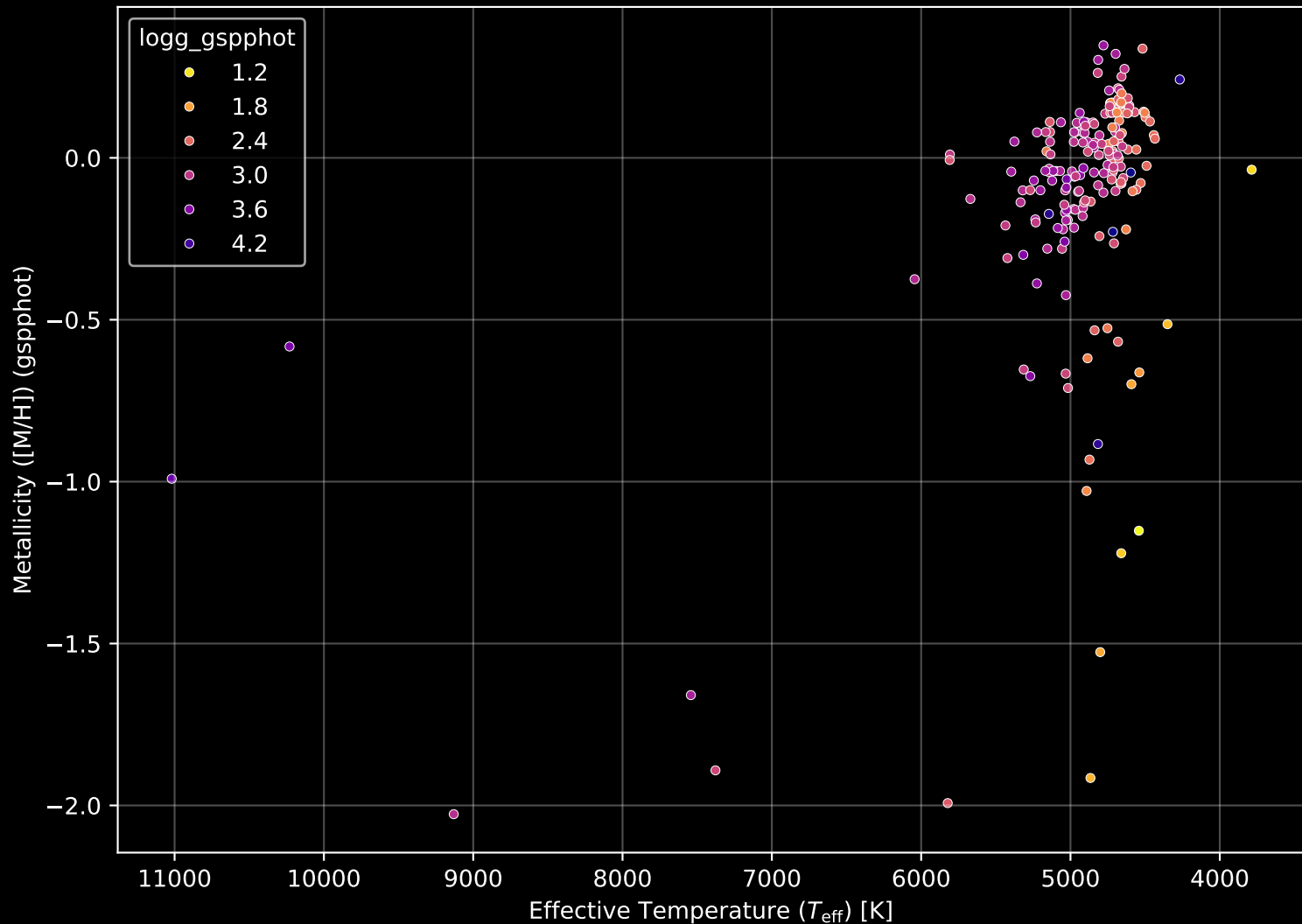
APOGEE DR17 Field: [296-06] Stellar Population Parameters (n= 193)
