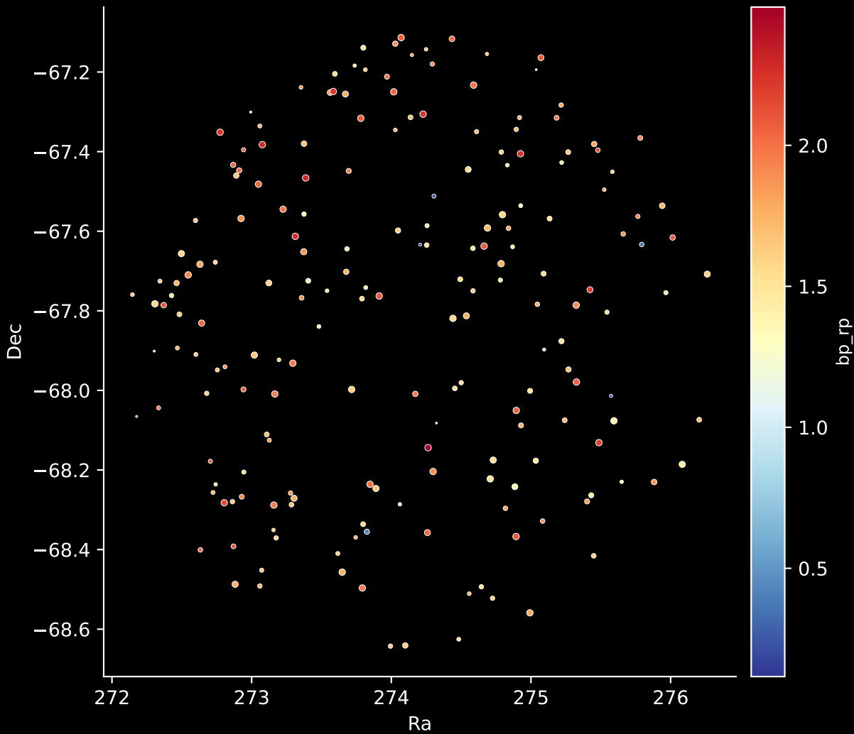
APOGEE DR17 Field: [296-06] Stars: 193
