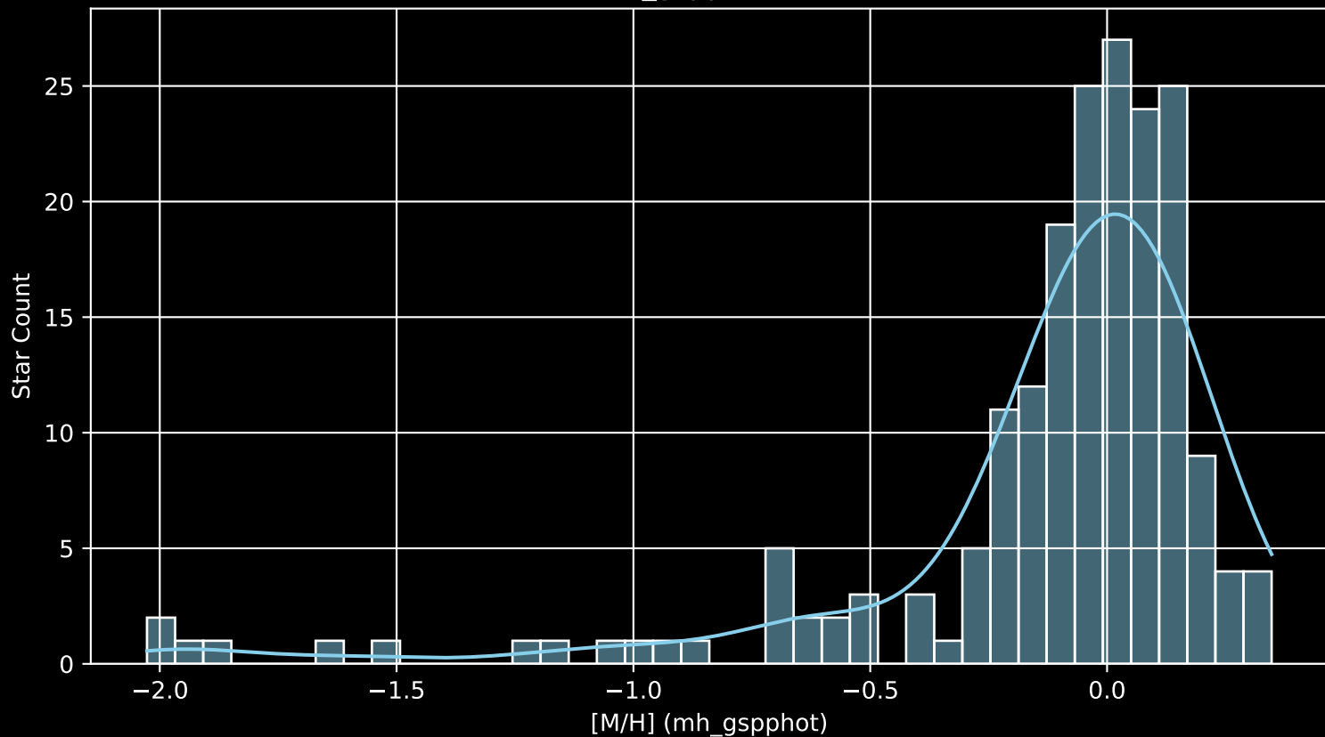
APOGEE DR17 Field: [296-06 [M/H] (mh_gspphot) (n= 193)
