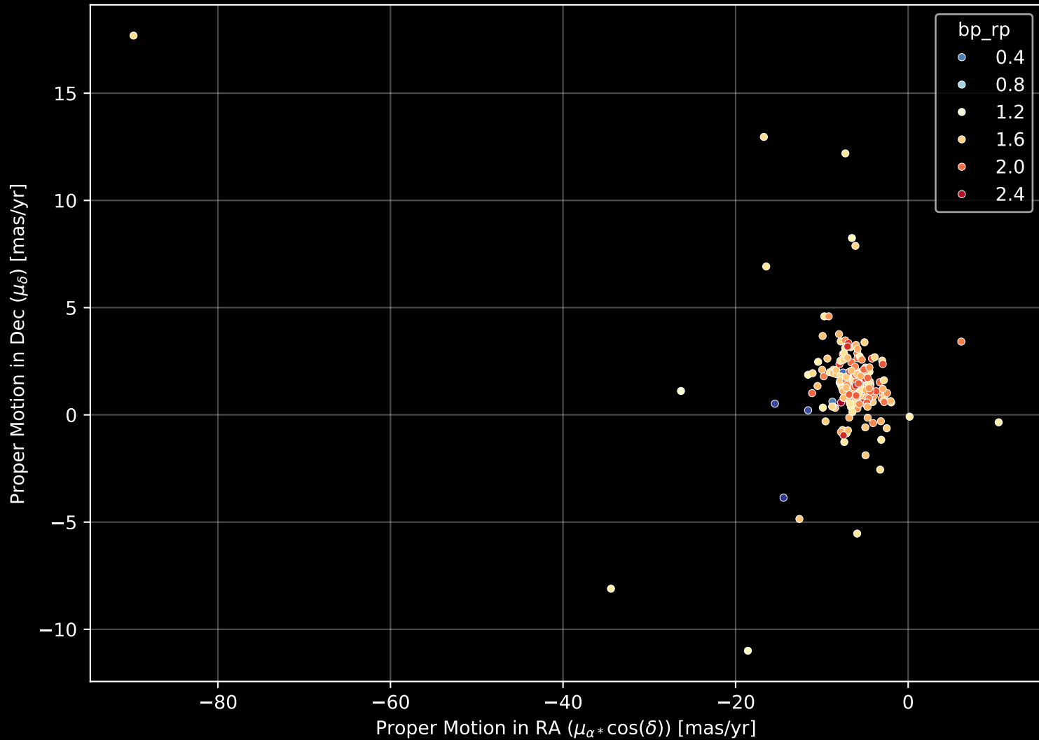
APOGEE DR17 Field: [296-06] Proper Motion Diagram (n= 193)
