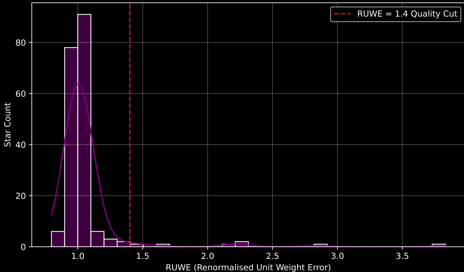
GAPOGEE DR17 Field [296-06] RUWE Distribution (n= 193)
