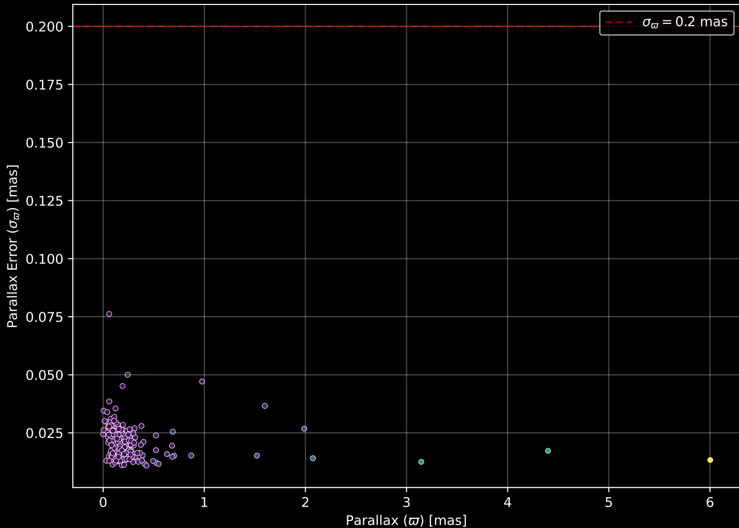
APOGEE DR17 Field: [296-06] Parallax Quality (n= 193)
